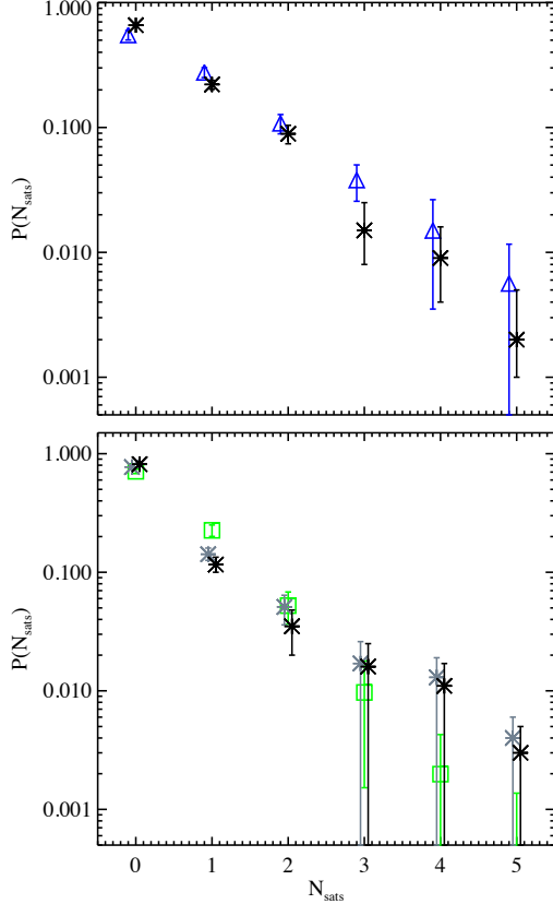
FIG. 8. — Comparisons between the P(N_{sats}) distribution of SMC-luminous satellites around MW-luminous hosts in the Bolshoi simulation and the observational results of L10. Top Panel: Comparison of the isotropic background subtraction model from L10. Black asterisks represent the abundances from SDSS hosts. The blue triangles denote the abundance of objects inside an aperture that most closely corresponds to the isotropic subtraction model: a fixed cylindrical aperture with radius 150 kpc and length 5.2 Mpc. Lower Panel: Same as the upper panel, but now comparing the annulus subtraction model from L10 (black and gray asterisks) to the simulation-equivalent of a fixed 150 kpc spherical aperture for identifying satellite galaxies around their hosts (green squares). For the L10 data, the black points represent our fiducial measurements, while the gray points add a systematic uncertainty to the background subtraction.
