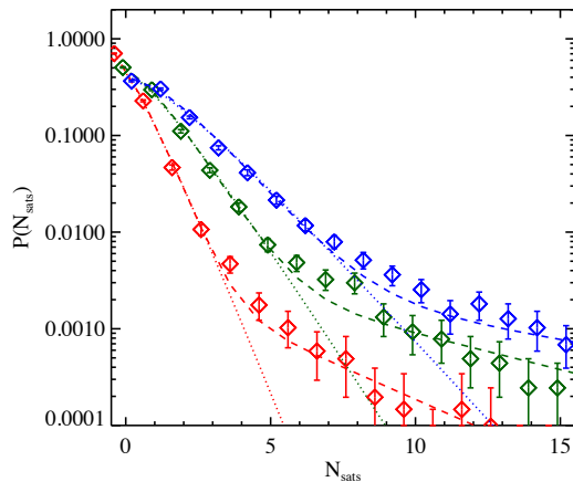
FIG. 12. — Probability of hosting N_{sats} satellite galaxies in a Milky Way-luminosity host, for various satellite selection criteria. The red, green, and blue points represent satellites brighter than M_r = -19.8, -18.2, and -16.8 . Dotted lines represent the best fit negative binomial distribution, while the dashed line shows the best fit negative binomial plus power-law distribution.
