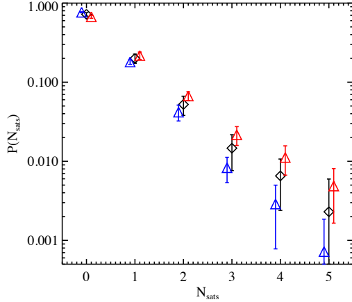
FIG. 11. — The probability distribution for a host galaxy to host N_S satellites within its virial radius split by environment. The black diamonds represent the distribution for all isolated hosts (and are identical to the black diamonds in Figure 7). The red and blue triangles represent the distribution for hosts in high and low density environments. Here, we use the total luminosity in galaxies brighter than M_r = -20.8 as our proxy for density.
